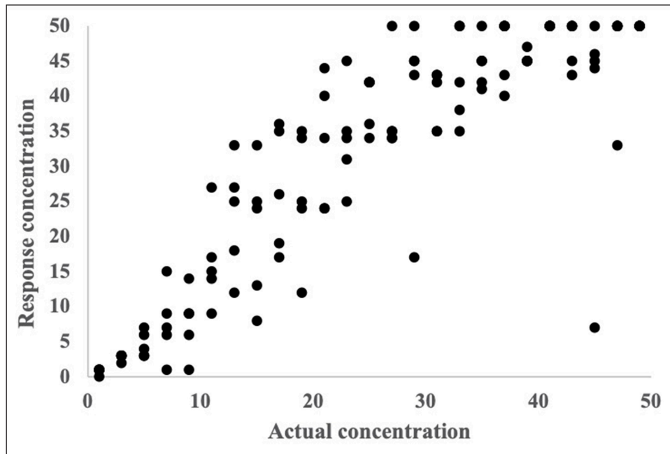
Figure 2 A scatter plot of data produced by continuous app users that compares the actual concentration of nitrate to the volunteers’ recorded values.
