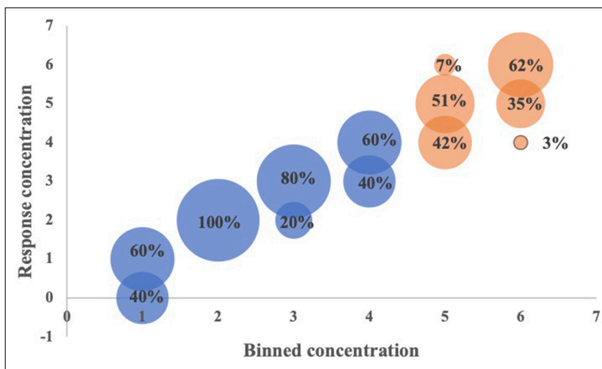
Figure 4 The relationship between nitrate concentrations and corresponding response categories produced by visual volunteers. The blue color corresponds to the samples in the lower range with smaller residuals and the orange corresponds to the samples in the higher range with residuals across three categories. The size of the circles provides a visual approximation of the proportion of samples that fall within each response concentration. In each case the total proportion equals 100%. The response concentration categories are defined by Hach as: 0 = 0ppm, 1 = 1ppm, 2 = 2ppm, 3 = 5 ppm, 4 = 10 ppm, 5 = 20 ppm, and 6 = 50 ppm.
