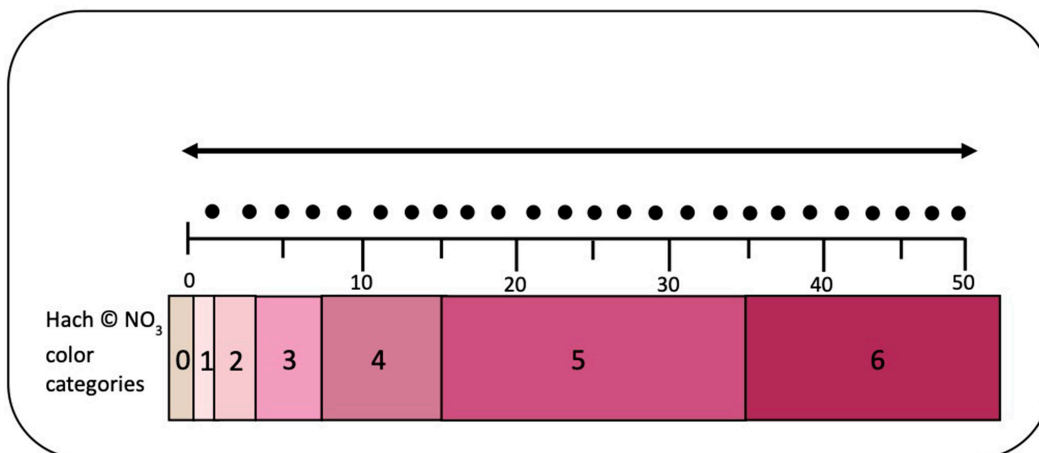
Figure 3 The dots represent continuous sample concentrations and their designated Hach© category bins. For example, concentrations that fall between 15.1 and 35.9 ppm (or mg/L) would be binned into category 5.
